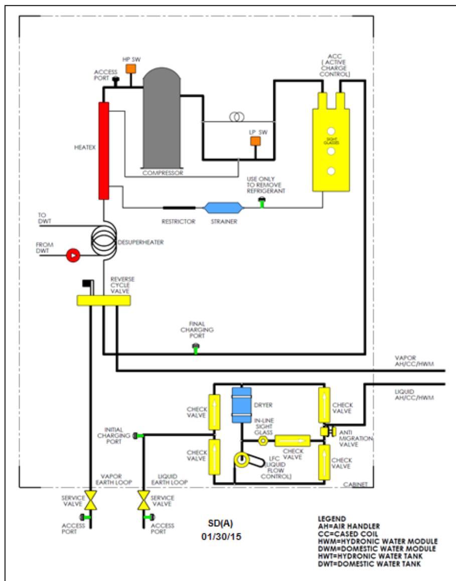
Figure 24. SD(A) Internal Flow Schematic
