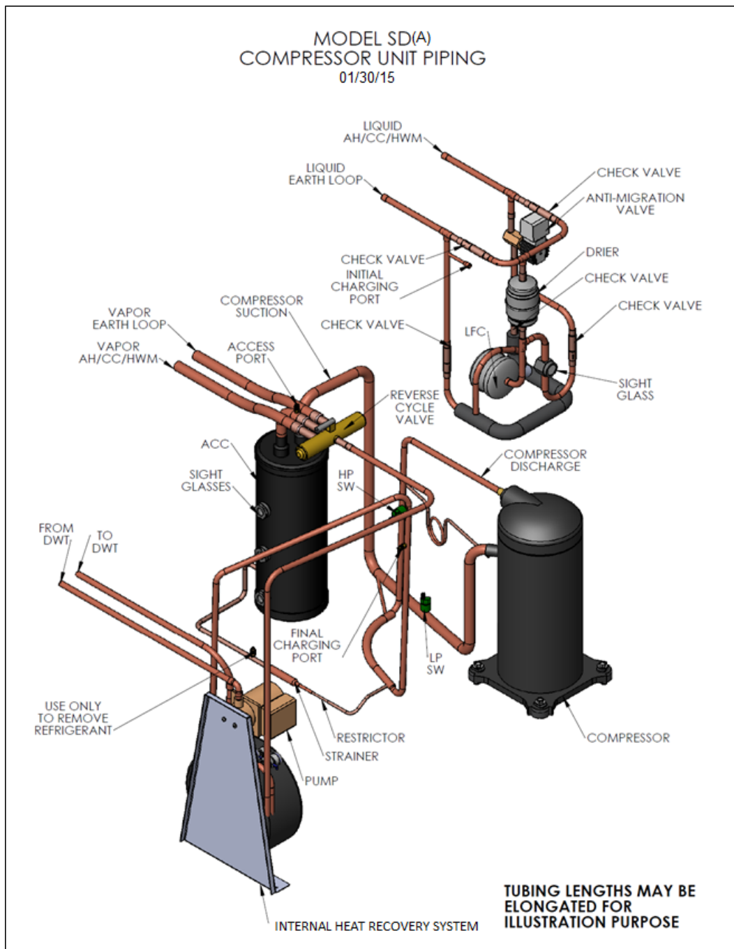
Figure 25. SD(A) Piping
