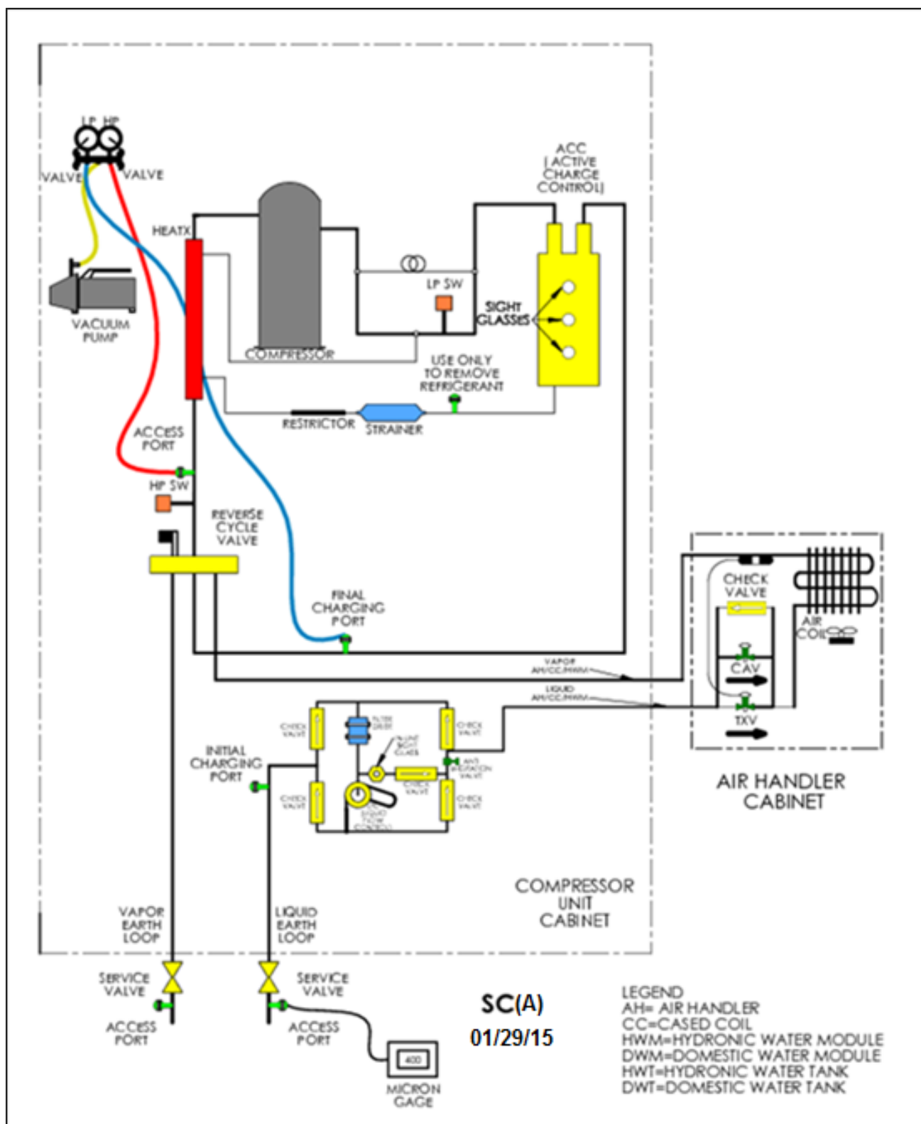
Figure 26. Evacuation of SD(A) System (SC(A) System Shown)
