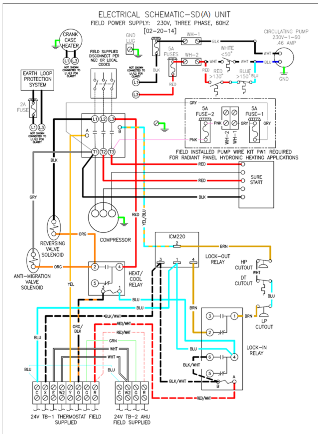
Figure 9b. SD(A) Compressor Unit Electrical Schematic Diagram, 230-3-60
