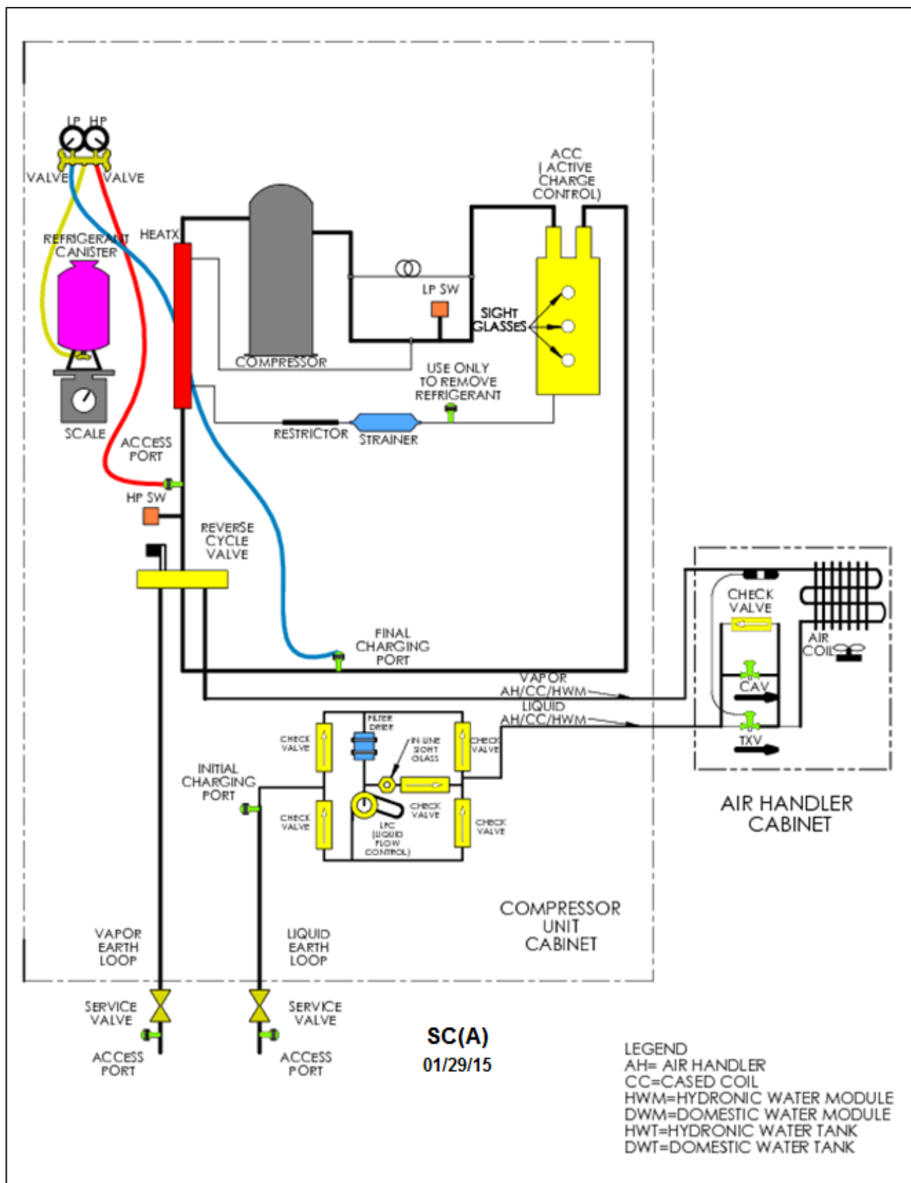
Figure 28. Final Charge of SD(A) System (SC(A) System Shown)
