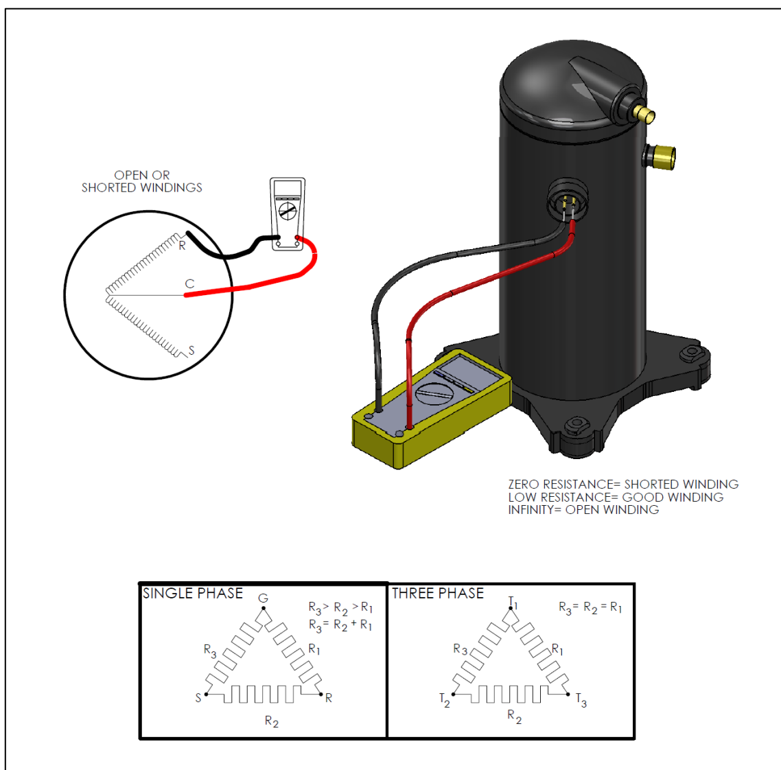
Figure 40. Compressor Motor Circuit Testing
