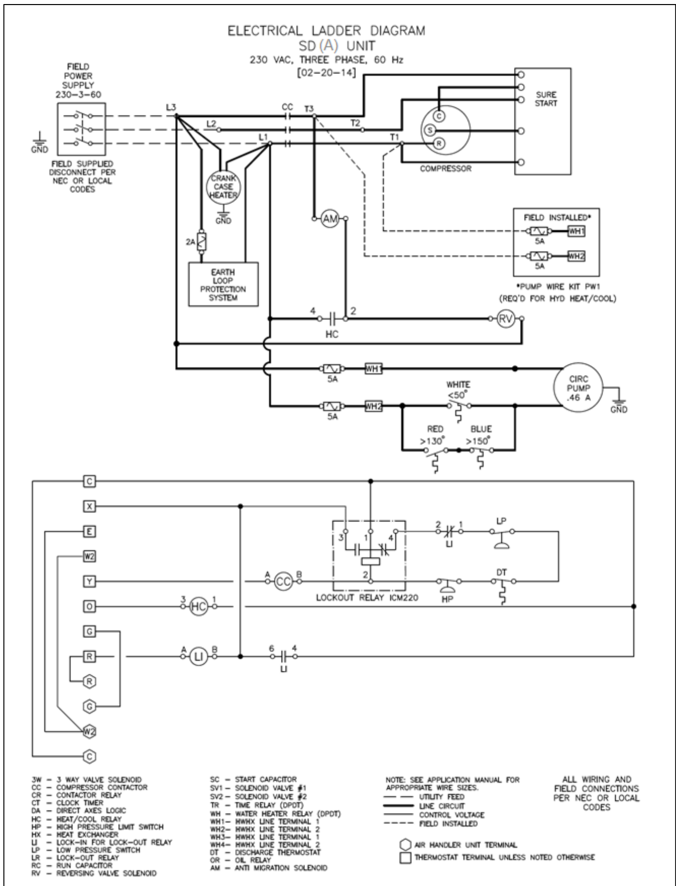
Figure 9a. SD(A) Compressor Unit Electrical Ladder Diagram, 230-3-60
