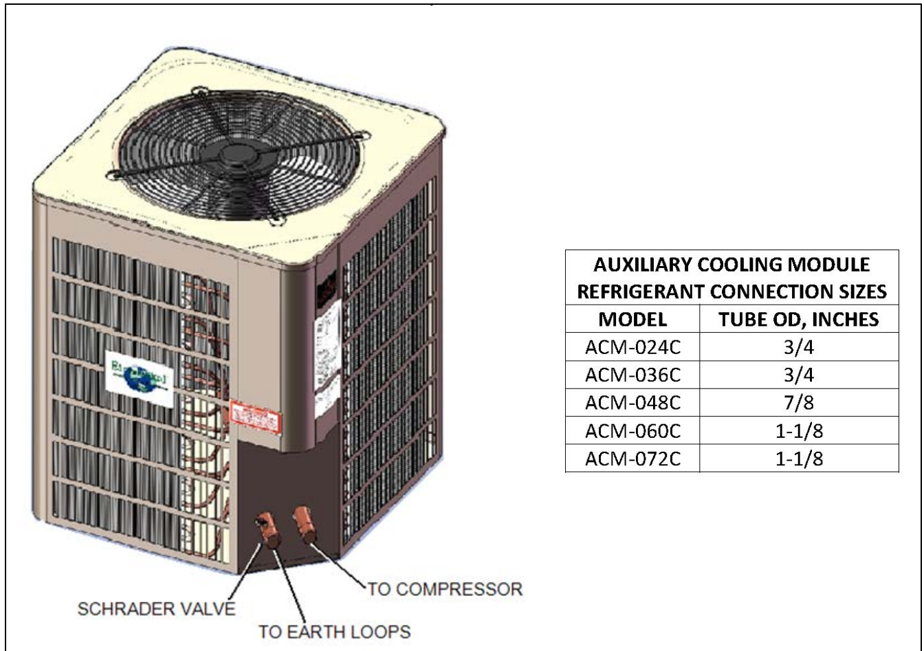
Figure 2. Auxiliary Cooling Module Refrigerant Connections
