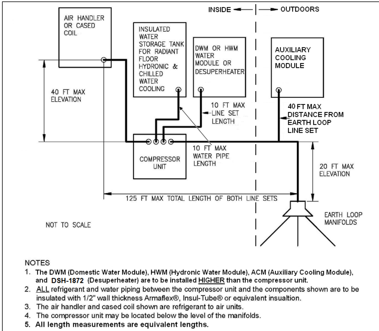
Figure 2. Auxiliary Cooling Module Placement in EarthLinked® System
